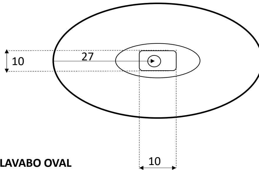
LAVABO OVAL VISTA INFERIOR
